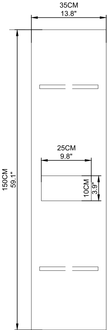
SIDE VIEW
